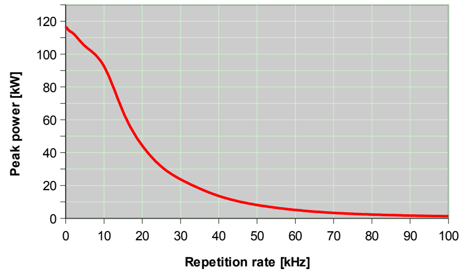
Sol 10 W 532 SS to 100 kHz: Peak Power
